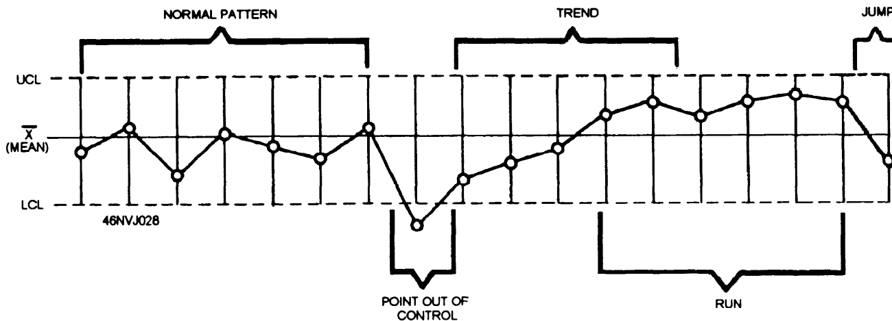
Figure 2-15.—Control chart interpretation.
